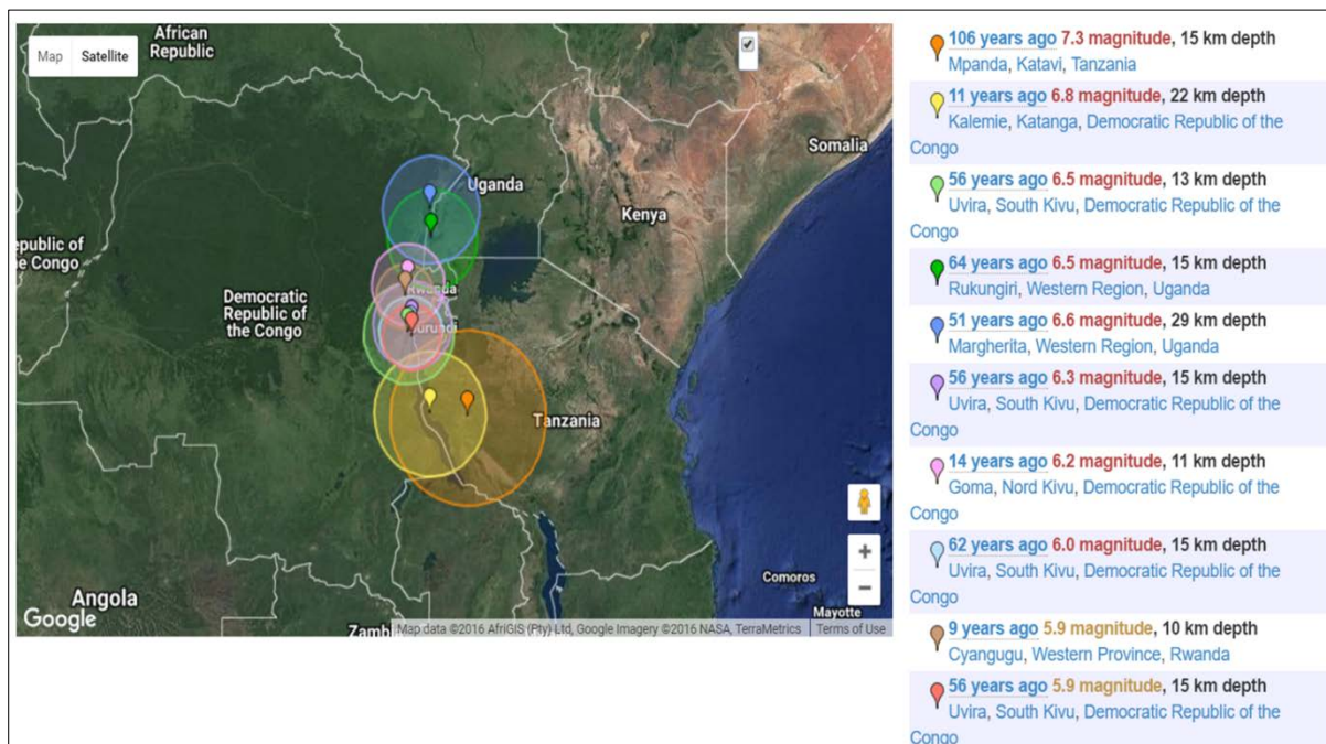
FIGURE 1: Major earthquake events along the Western branch of the EARS
