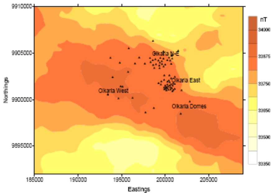
FIGURE 4: Map showing total magnetic intensity over Olkaria (Mariita, 1995)
