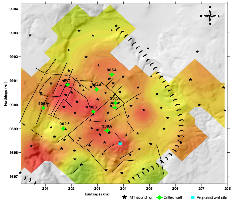
FIGURE 1: MT resistivity iso-anomaly map at 700 masl (m above sea level) of Domes area.
