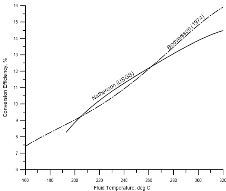
FIGURE 3: Correlation between thermal conversion efficiency and reservoir temperatures (From Nathenson, 1975 and Bodvarsson, 1974).
