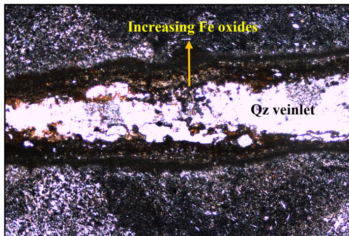
FIGURE 20: Quartz veinlet and Fe oxides increased towards the rim and groundmass (sample 291). Thin section viewed in plane polarized light
