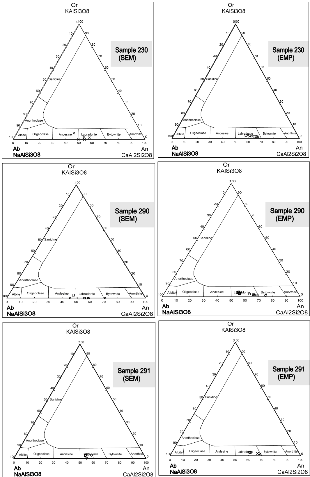
FIGURE 26: Plagioclase composition in the inner hornfels zone determined by both SEM/EMP, data from Appendix II and III. Xs are plagioclase composition in the vesicle centre. Circles are the composition at the margin while squares are at the groundmass
