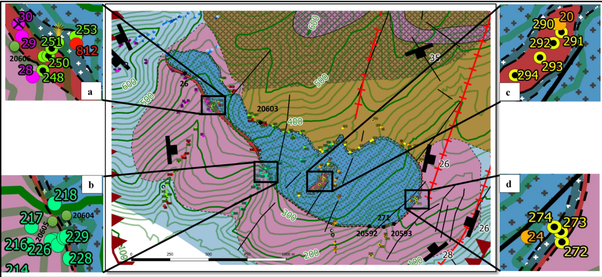
FIGURE 10: Geological map of the Hrossatungur gabbro and surroundings. Small squares enclose the locations of sampling profiles (a), (b), (c) and (d) while A, B, C and D subfigures show the analytical numbers referring of as listed in appendices. The varying colours of the numbers represent different field days. Sample location 272, represents a profile containing four samples (id of the four samples)
