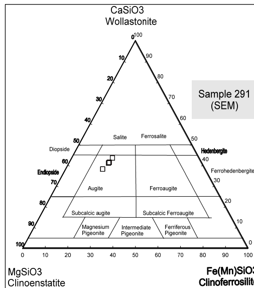
FIGURE 22: Pyroxene composition in the inner hornfels contact zone determined by both SEM and EMP in term of Ca-Mg-Fe element, data from Appendices II and III. Xs are pyroxene composition at the vesicle centre. Circles are the composition at the margin while squares are at groundmass
