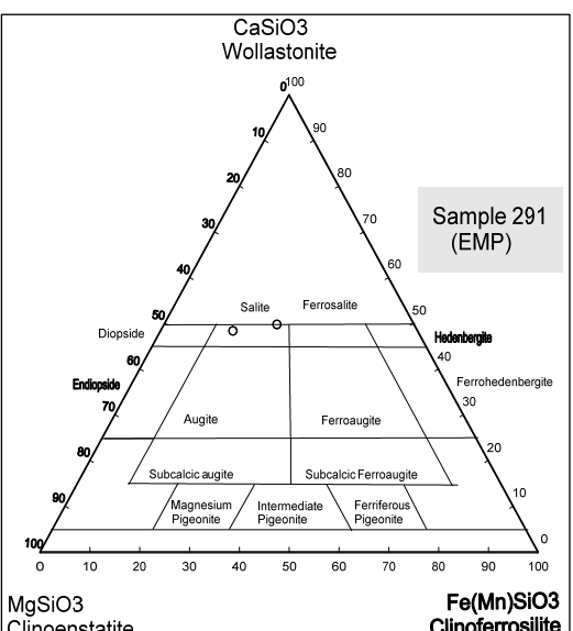
FIGURE 22: Pyroxene composition in the inner hornfels contact zone determined by both SEM and EMP in term of Ca-Mg-Fe element, data from Appendices II and III. Xs are pyroxene composition at the vesicle centre. Circles are the composition at the margin while squares are at groundmass
