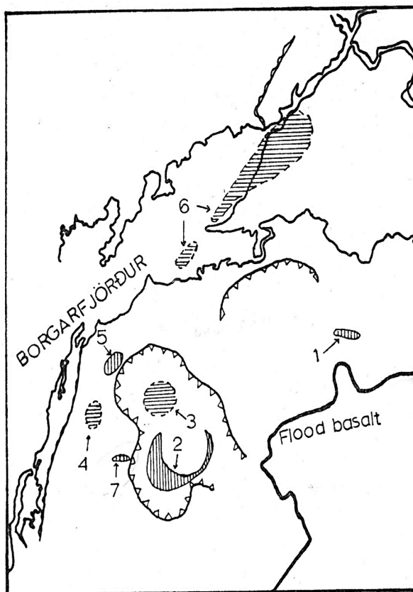
FIGURE 3: Location of larger intrusions in the central volcano. Solid lines show exposed intrusions, while intrusions outlined by broken lines are proposed based on indirect evidence. Intrusion marked 2 is the Hrossatungur gabbro (Franzson, 1979)
