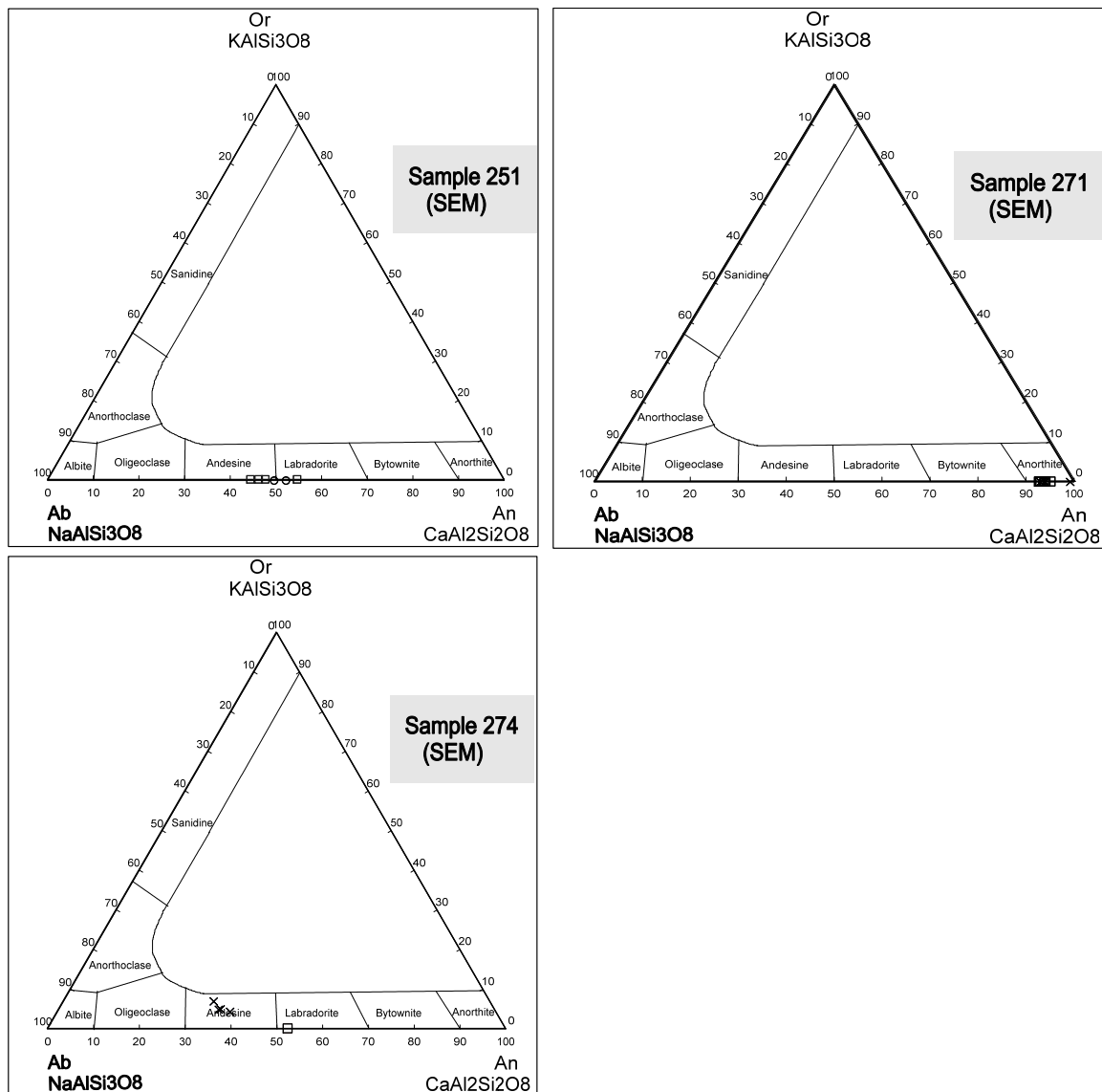
FIGURE 27: Plagioclase composition in the inner hornfels contact zone determined by only SEM in terms of An-Ab-Or elements, data from Appendix II. Xs are plagioclase composition at the vesicle centre. Circles are the composition at the margin while squares are at the groundmass
