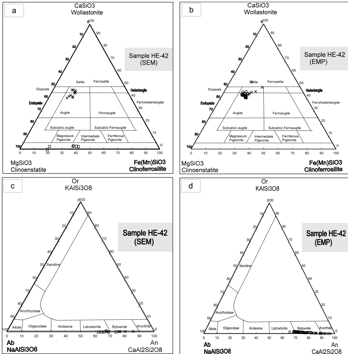
FIGURE 41: Pyroxene and plagioclase compositions in the hornfels zone in well HE-42 (Hellisheidi) determined by SEM/EMP in terms of Ca-Mg-Fe and Ab-An-Or components, data from appendix II and III. Xs are compositions at the vesicle centre. Circles are the composition at the margin while squares are within the groundmass
